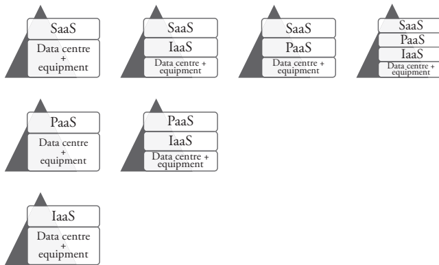
Figure 1.1 Cloud layers—different architectures
